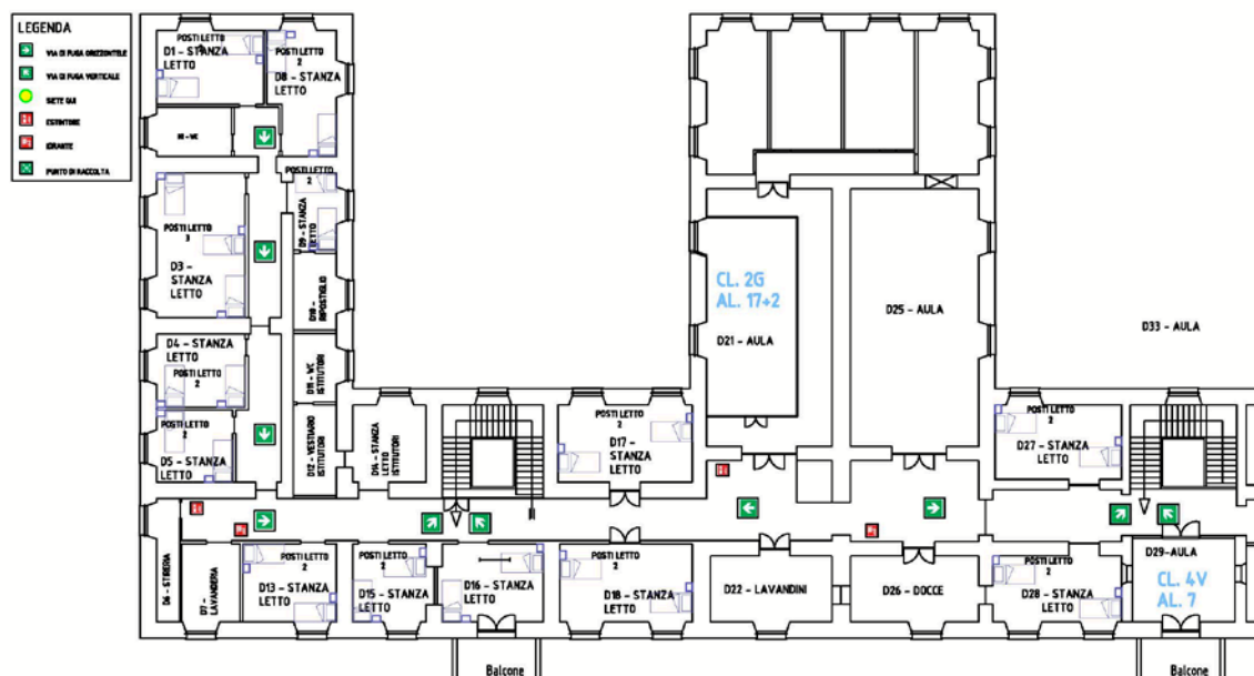
PIANTA PIANO CONVITTO
